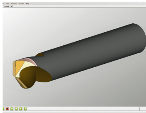
/////// SIMULATION ERODIEROPERATION Erodieren von PKD
